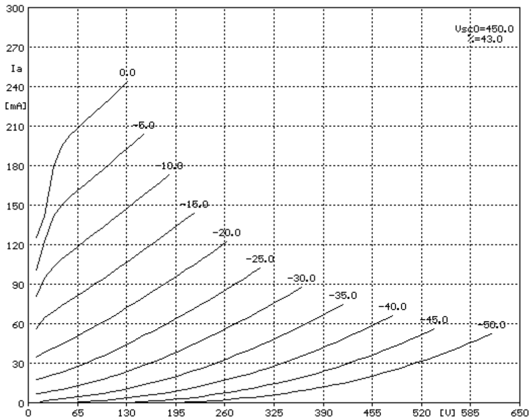
KT66 penthode mode connection.
